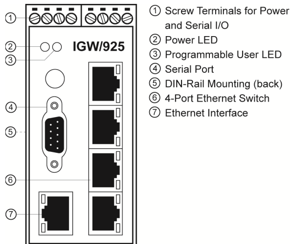
Basic hardware interfaces of the IGW/925
